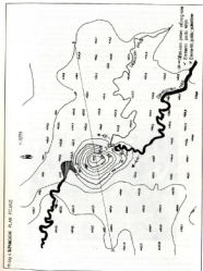
Figure 4 – Svalbard Plate Region
